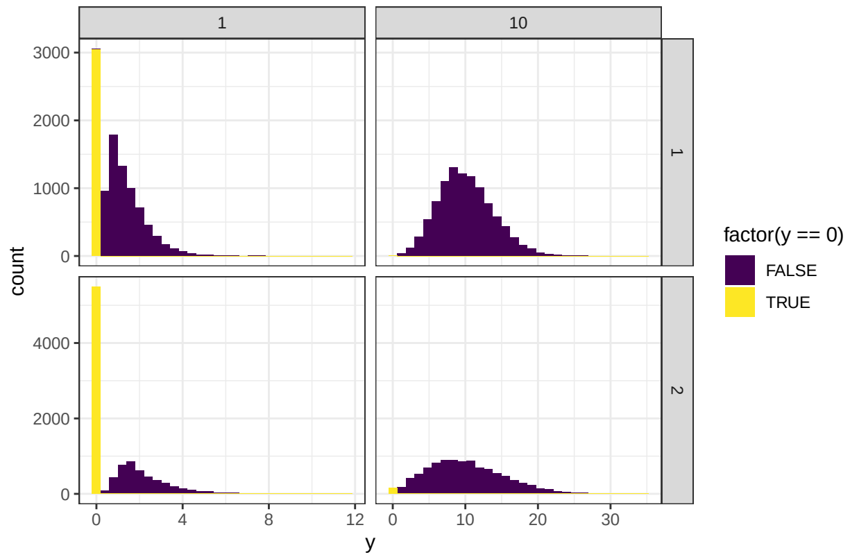
Tweedie with zero inflation
