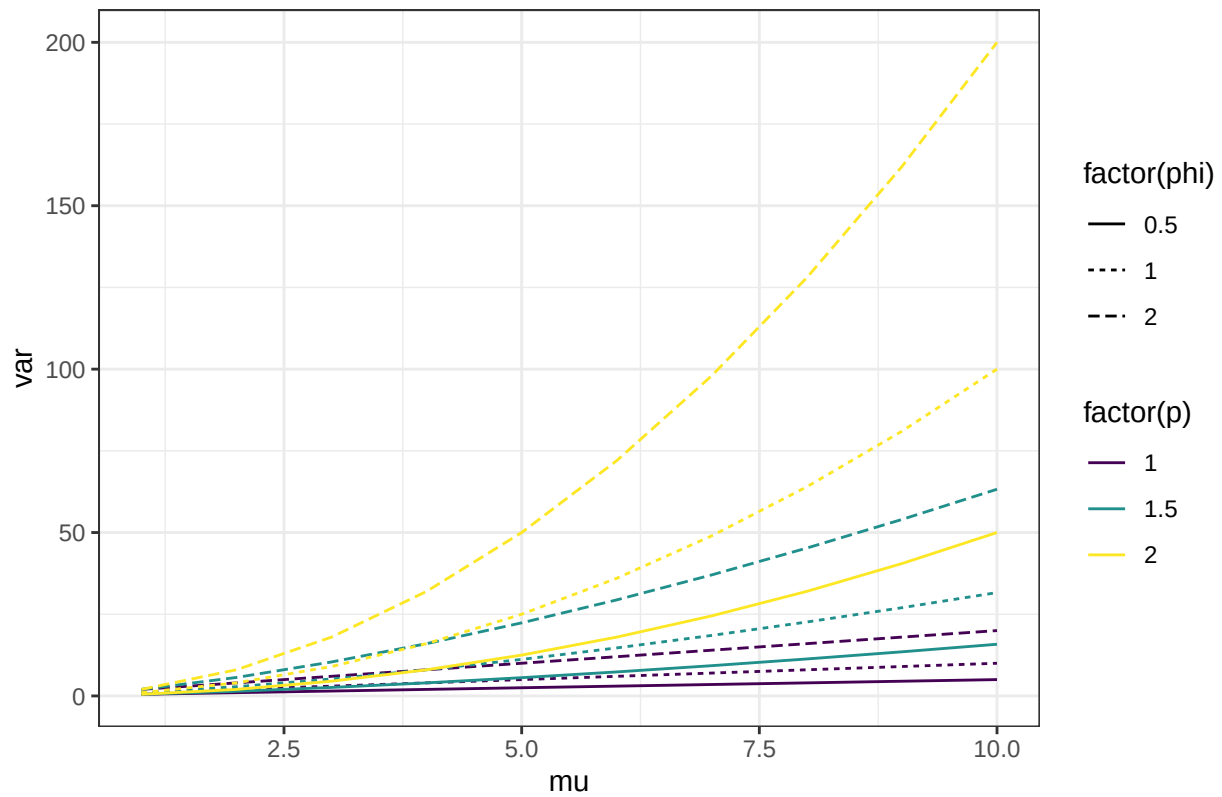
Variance with mean, p , and \phi
